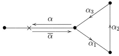
Figure 2. A bounce path \alpha\alpha_3\alpha_2\alpha_1\bar{\alpha} with n = 3 .
