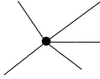
Figure 1. A star.
